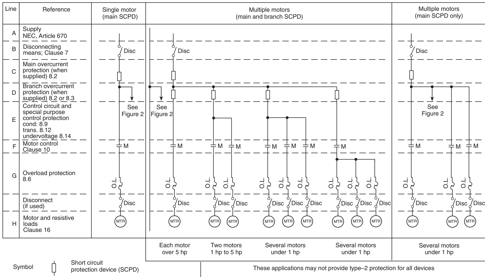
Figure 1 — One line representation of electrical system power distribution
