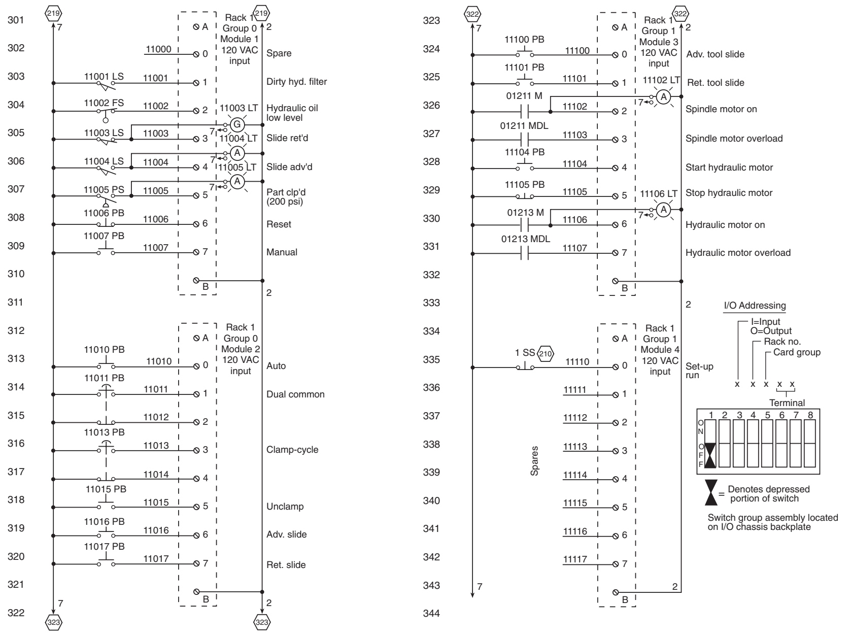
Figure D.6 P.C. input wiring diagram
