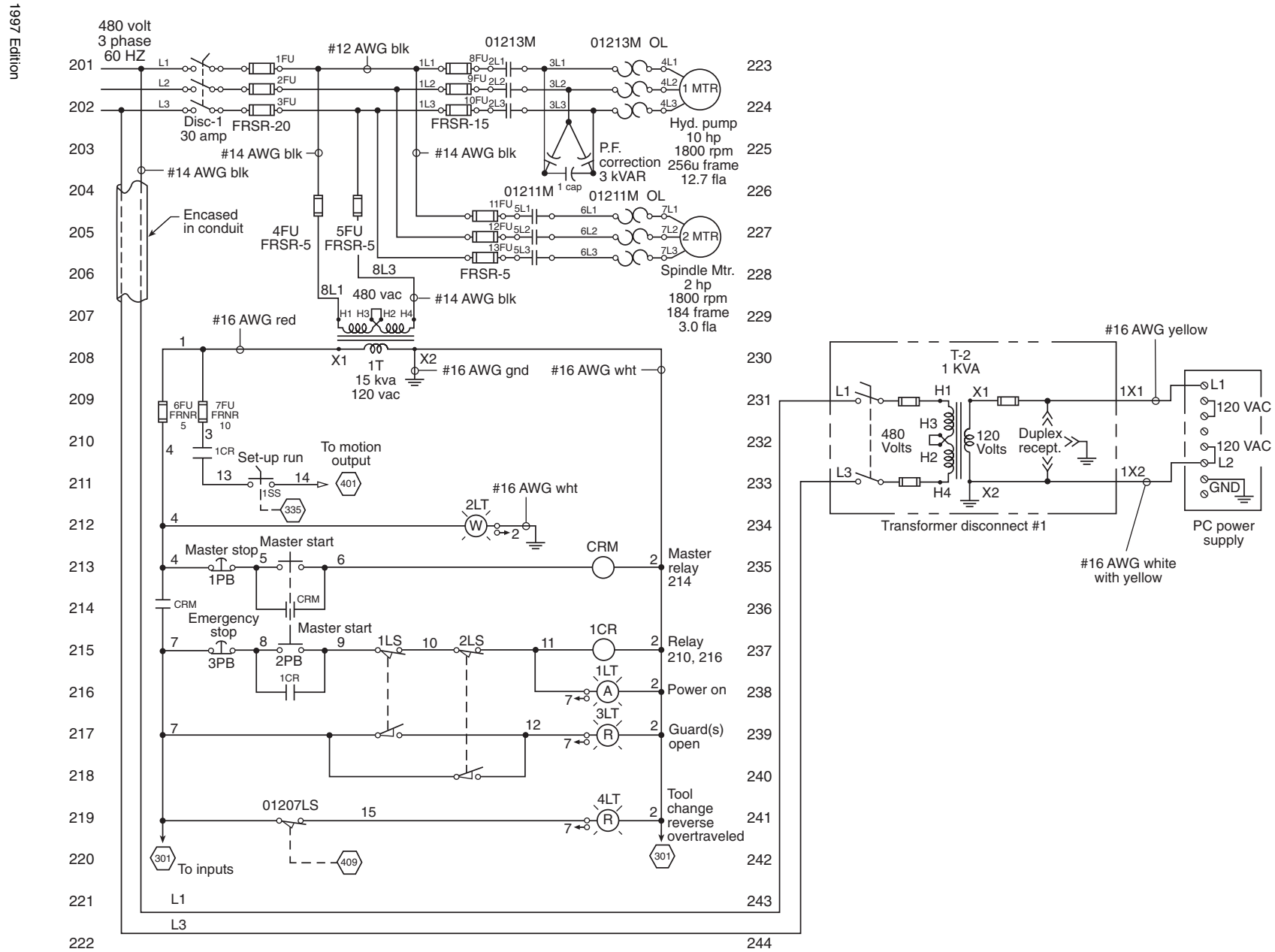
Figure D.5 P.C. hardware electrical schematic
