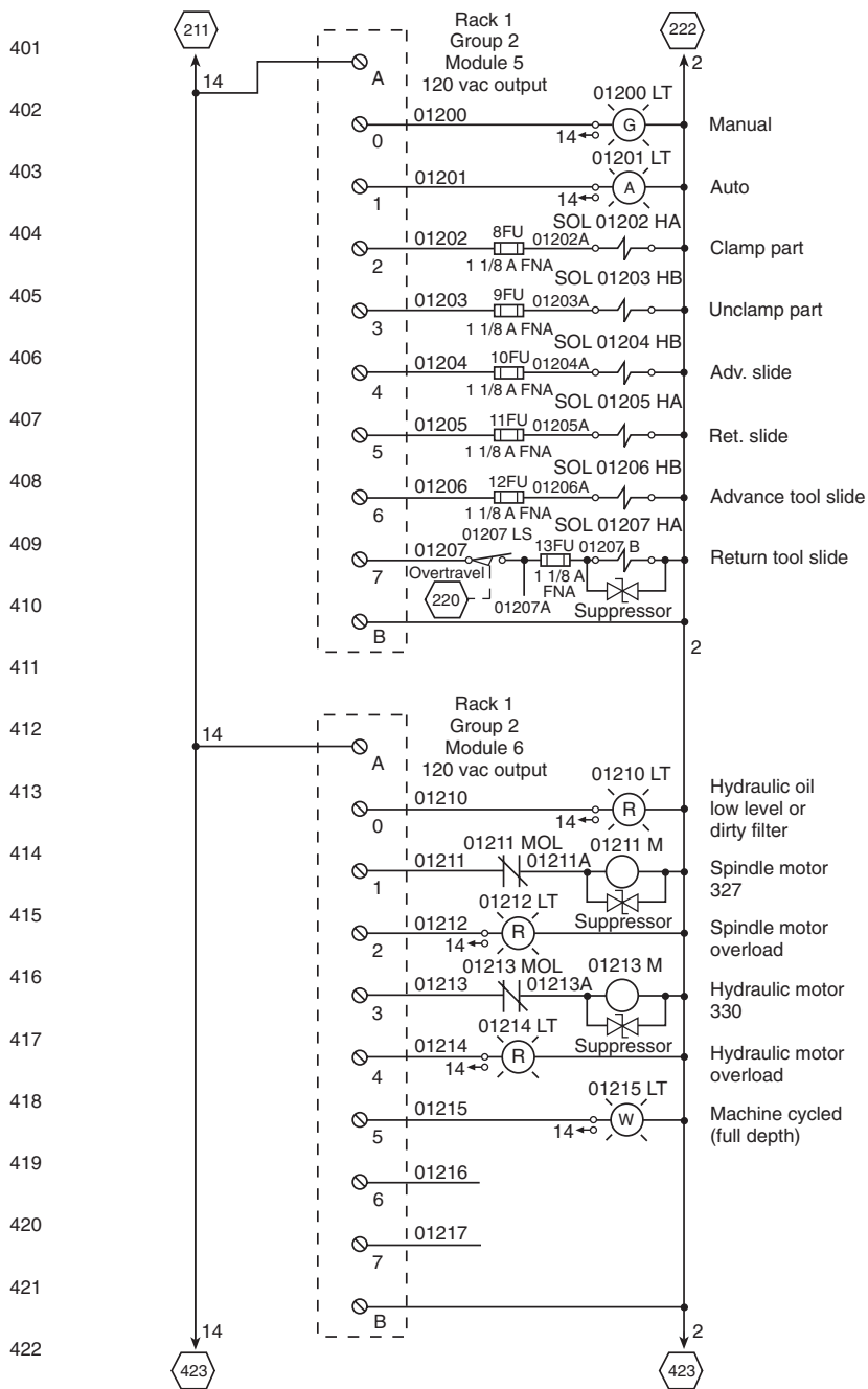
Figure D.7 P.C. output wiring diagram
